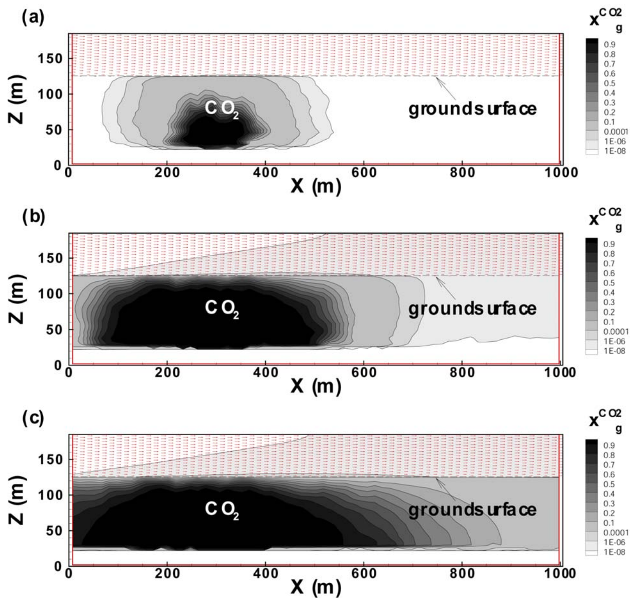
Figure 4.14. Coupled \text{CO}_2 subsurface migration and surface-layer mixing at 1, 10, and 200 years after \text{CO}_2 migration begins for wind velocity of 3 \text{ m s}^{-1} and permeability realization A in a horizontal system.
