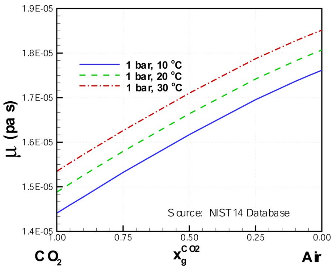
Figure 3.2. Viscosity as a function of concentration (mole fraction) in the system \text{CO}_2 -air.
