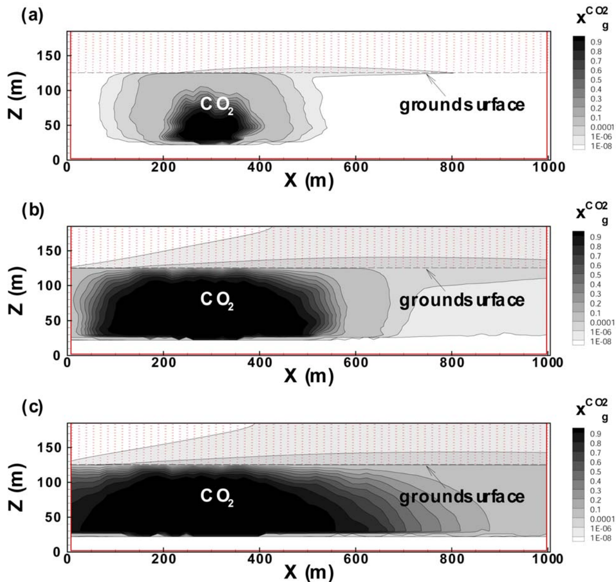
Figure 4.15. Coupled \text{CO}_2 subsurface migration and surface-layer mixing at 1, 10, and 200 years after \text{CO}_2 migration begins for wind velocity of 1 \text{ m s}^{-1} and permeability realization A in a horizontal system.
