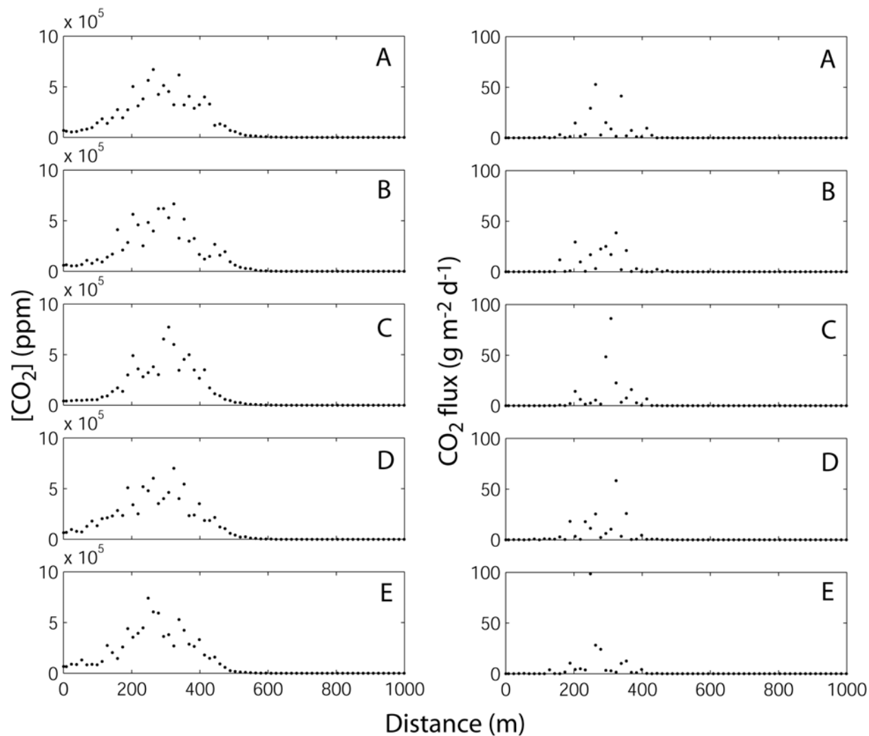
Figure 4.12. Horizontal profiles of shallow subsurface \text{CO}_2 concentration ( [\text{CO}_2] , 3 m depth) and surface \text{CO}_2 flux for high ( 576 \text{ g m}^{-2} \text{d}^{-1} ) \text{CO}_2 source flux, heterogeneous isotropic permeability realizations A-E, and t = 200 years.
