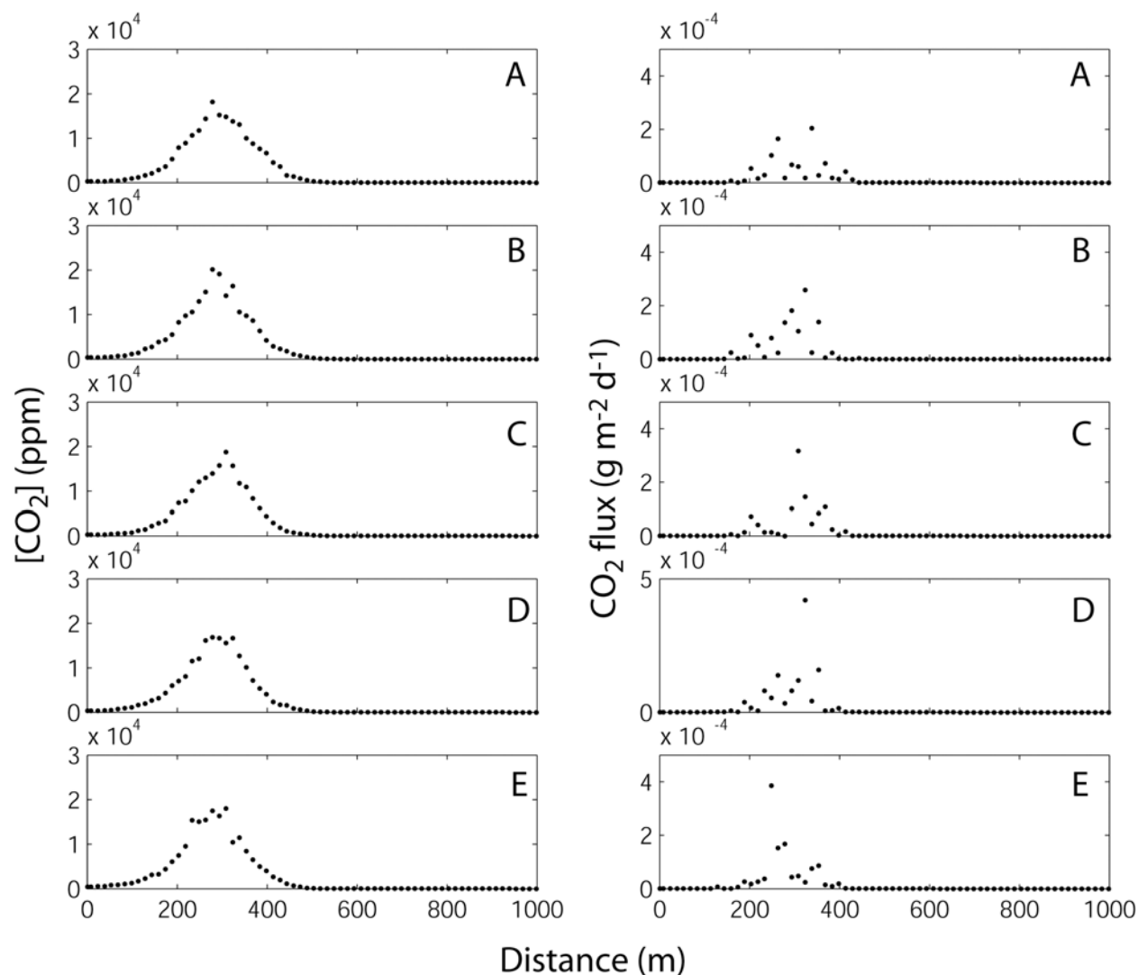
Figure 4.10. Horizontal profiles of shallow subsurface \text{CO}_2 concentration ( [\text{CO}_2] , 3 m depth) and surface \text{CO}_2 flux for low ( 5.76 \text{ g m}^{-2} \text{ d}^{-1} ) \text{CO}_2 source flux, heterogeneous isotropic permeability realizations A-E, and t = 200 years.
