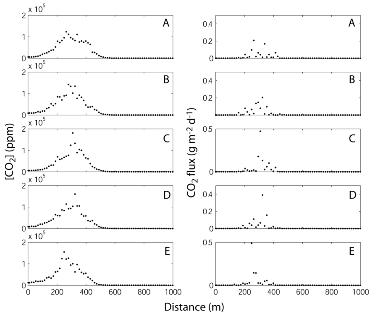
Figure 4.11. Horizontal profiles of shallow subsurface \text{CO}_2 concentration ( [\text{CO}_2] , 3 m depth) and surface \text{CO}_2 flux for medium ( 57.6 \text{ g m}^{-2} \text{d}^{-1} ) \text{CO}_2 source flux, heterogeneous isotropic permeability realizations A-E, and t = 200 years.
