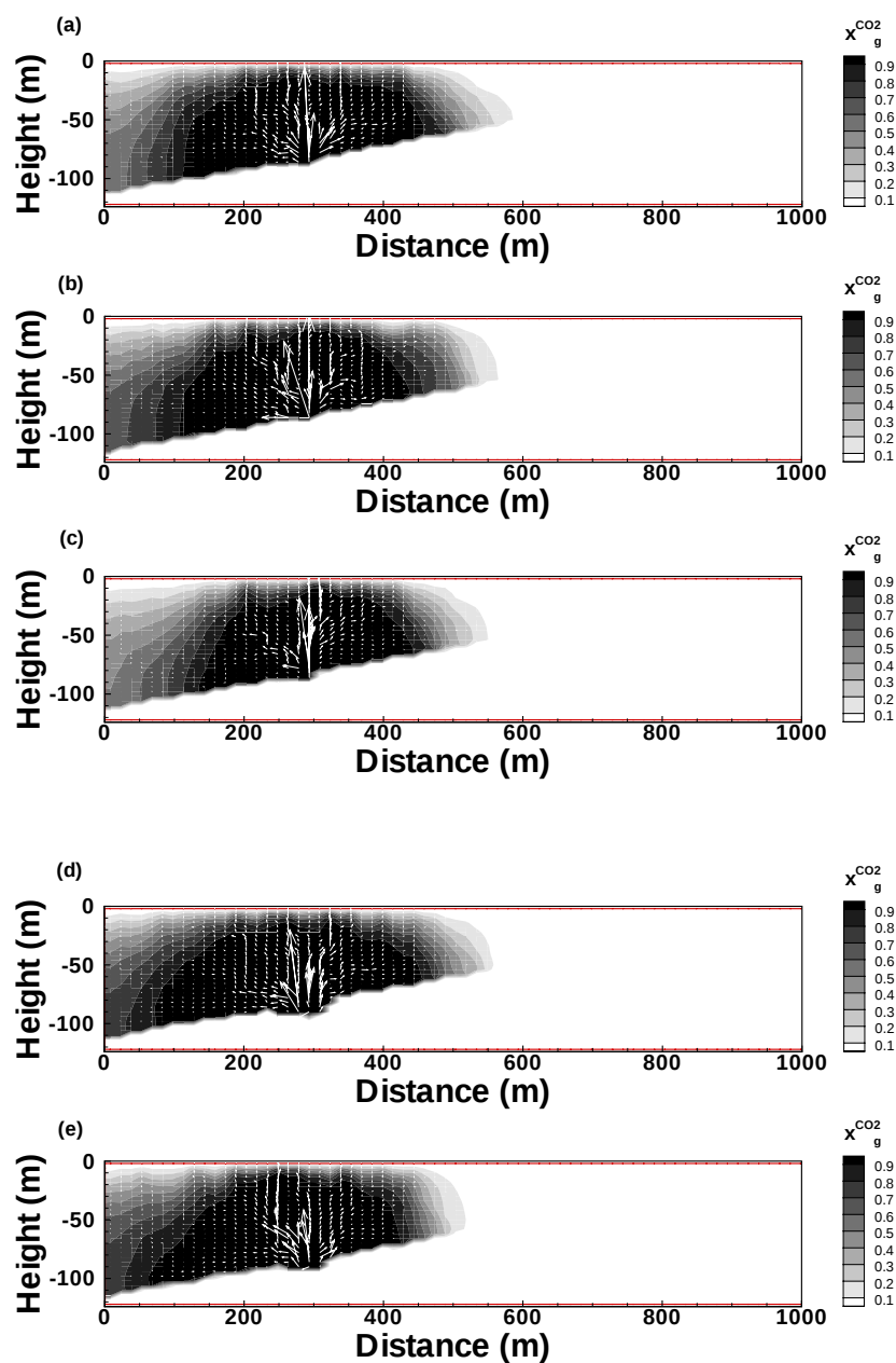
Figure 4.8. Subsurface CO 2 concentrations (mole fraction) at t = 200 years for five permeability realizations (A–E) and high CO 2 source flux ( 576 \text{ g m}^{-2} \text{ d}^{-1} ).
