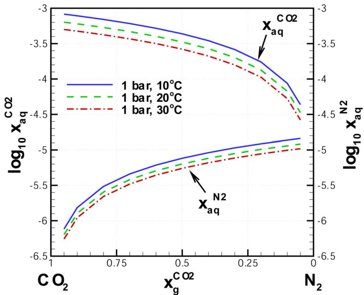
Figure 3.3. Solubility of \text{CO}_2 and \text{N}_2 in water (mole fraction) in gas and aqueous phases.
